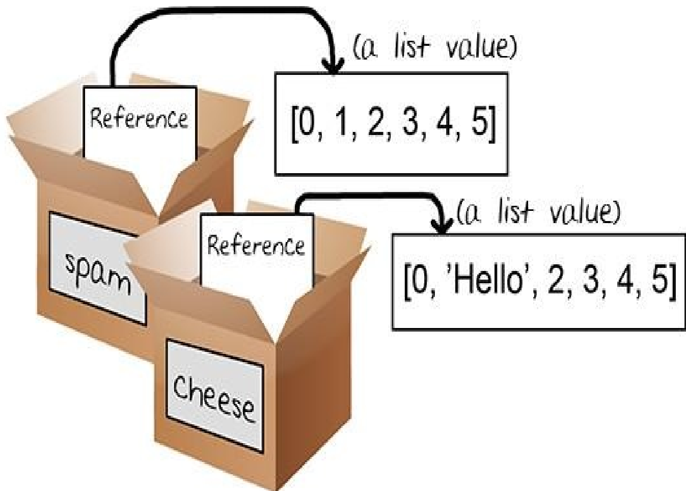
Figure 10-4. Two variables each storing references to two different lists.
