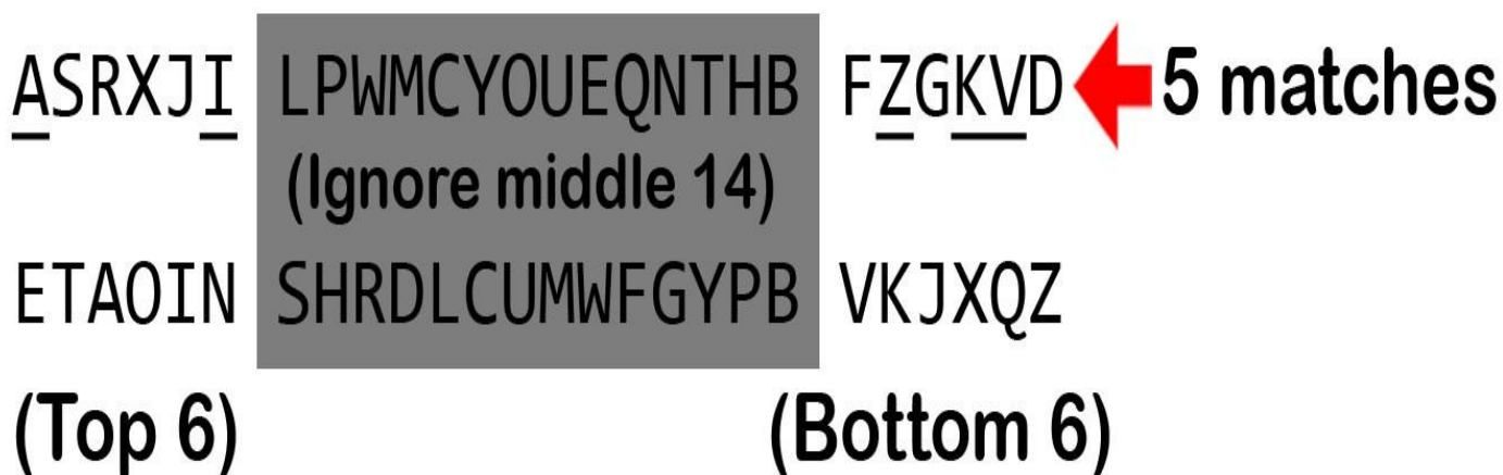
Figure 20-3. How the frequency match score of ASRXJILPWCYOUQNTHEBFZGKVD is calculated.
