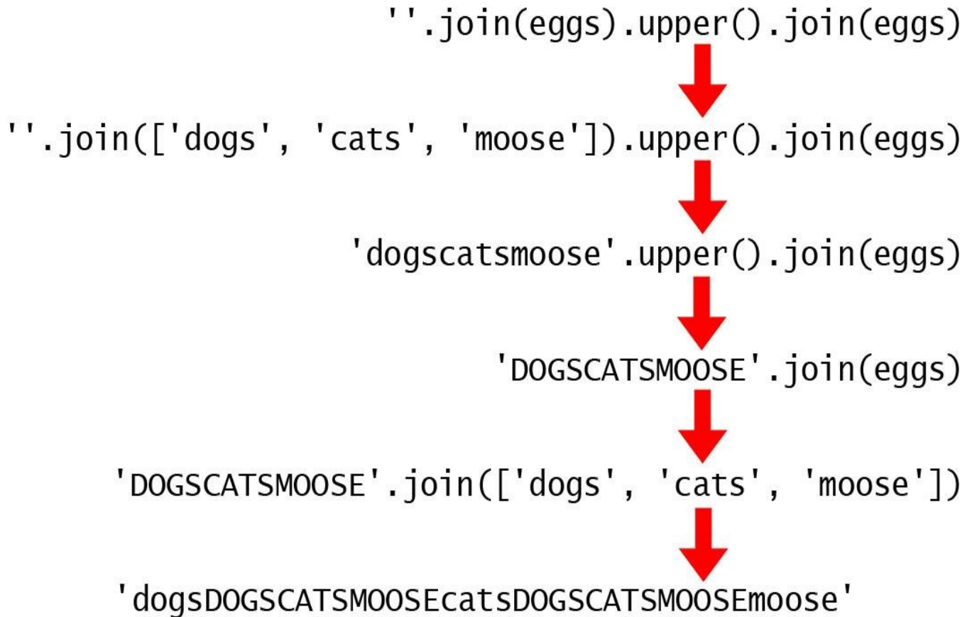
Figure 8-4. The steps of evaluation for ".join(eggs).upper().join(eggs)
