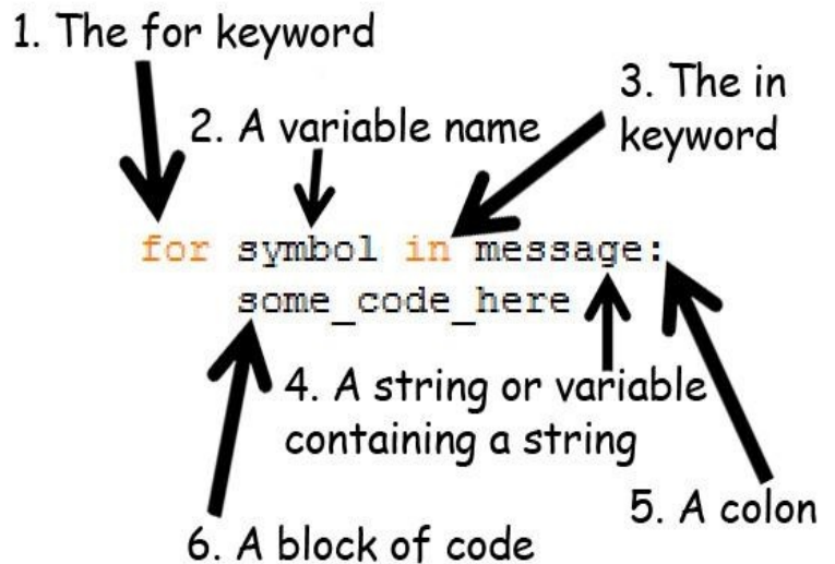
Figure 6-1. The parts of a for loop statement.
