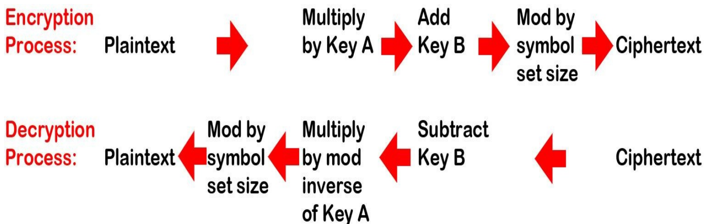
Figure 14-8. The encryption and decryption are mirrors of each other.
