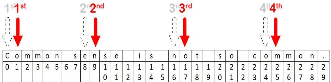
Figure 8-3. Arrows pointing to to what message[pointer] refers to during the second iteration of the for loop when col is set to 1.
