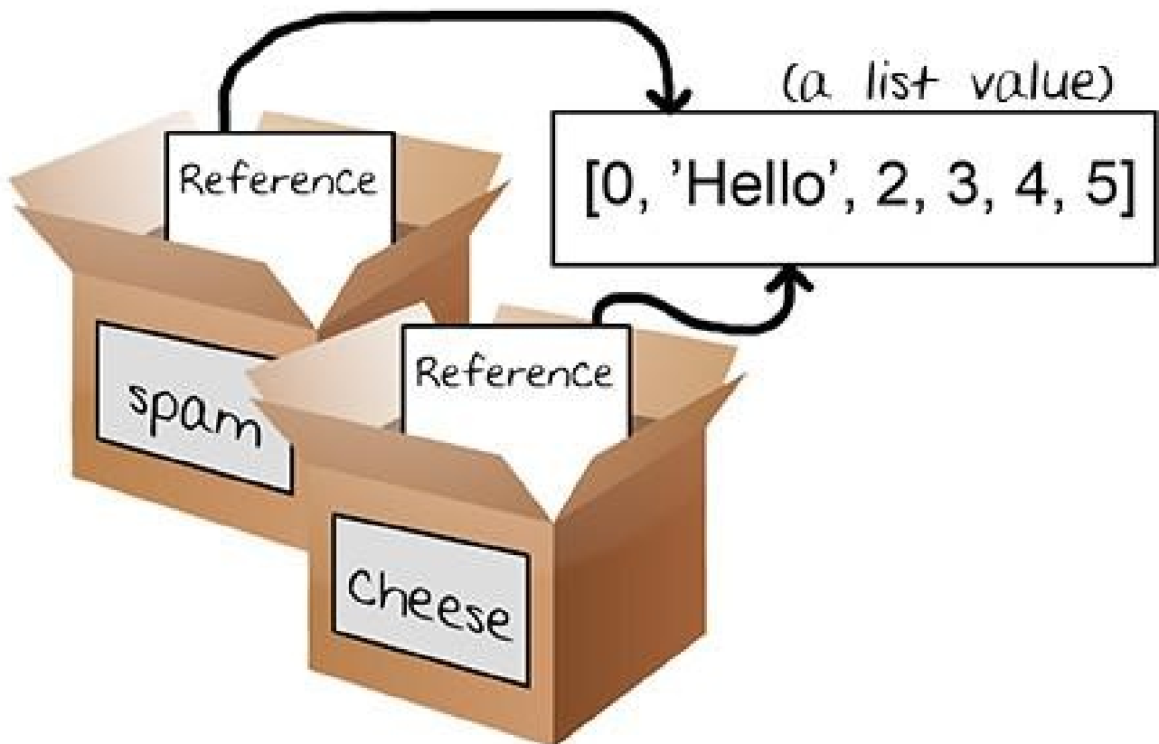
Figure 10-3. Changing the list changes all variables with references to that list.
